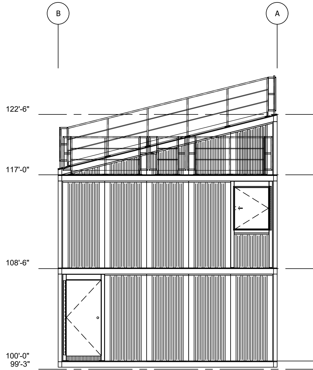
D RIGHT SIDE ELEVATION Scale: NTS
