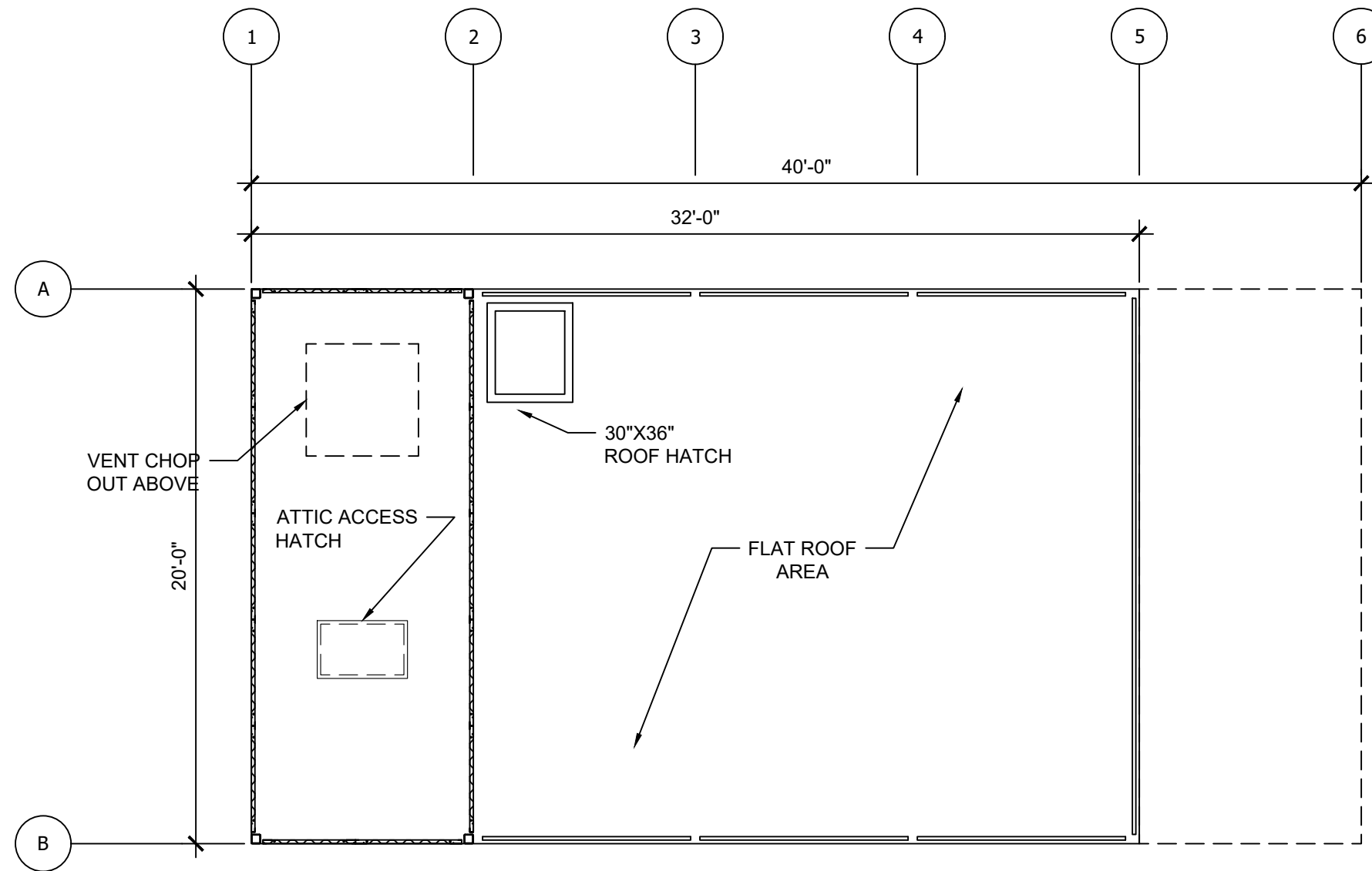
3 ROOF (ATTIC) LAYOUT Scale: NTS
