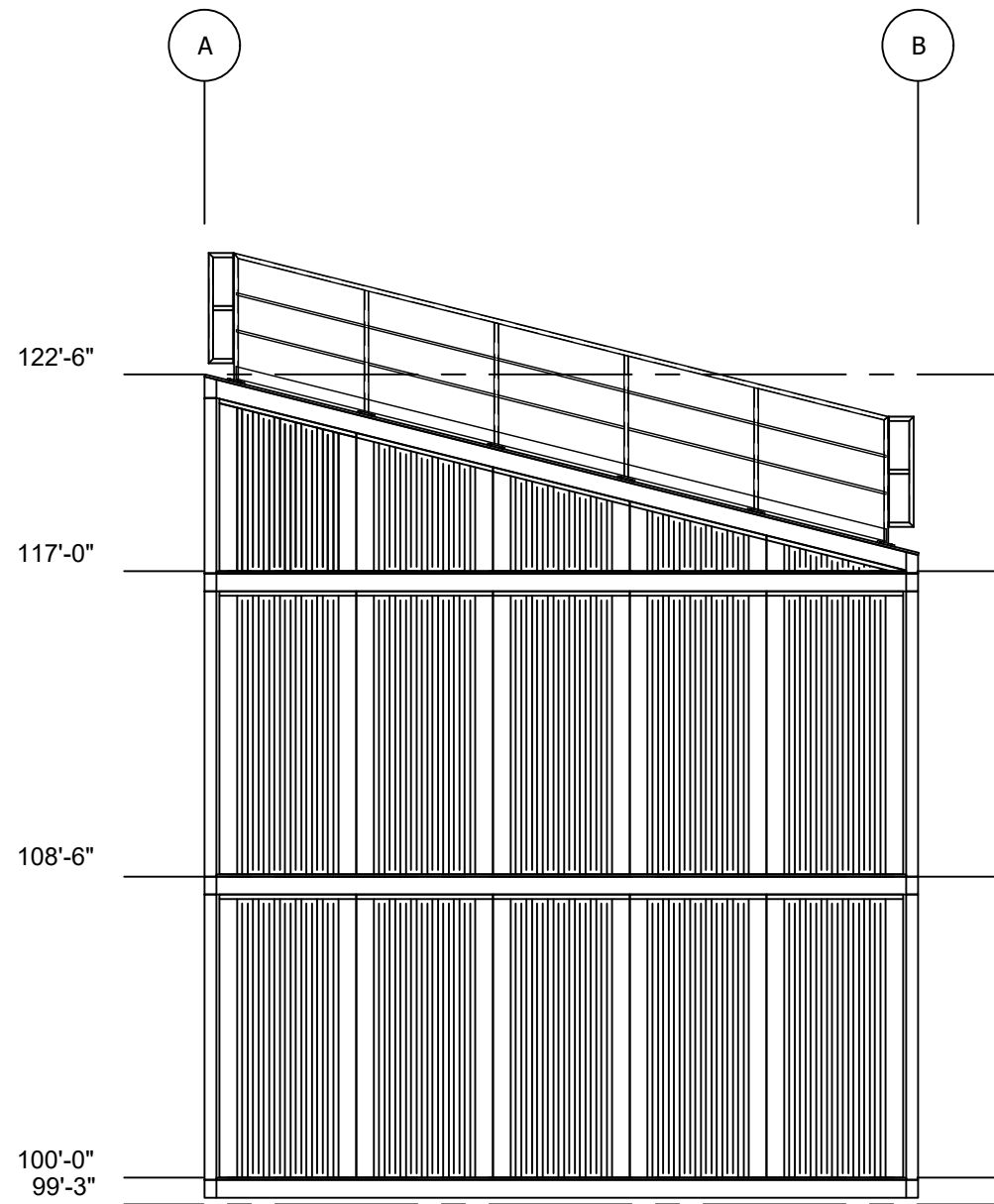
B LEFT SIDE ELEVATION Scale: NTS
