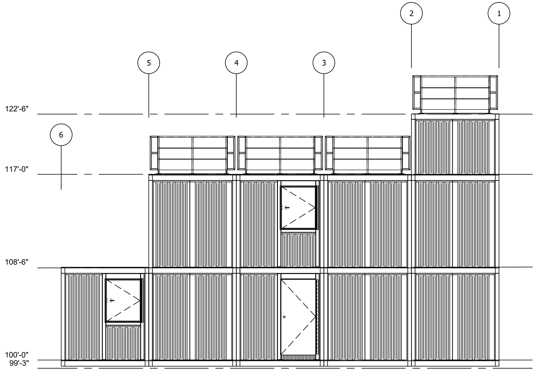
C REAR SIDE ELEVATION Scale: NTS
