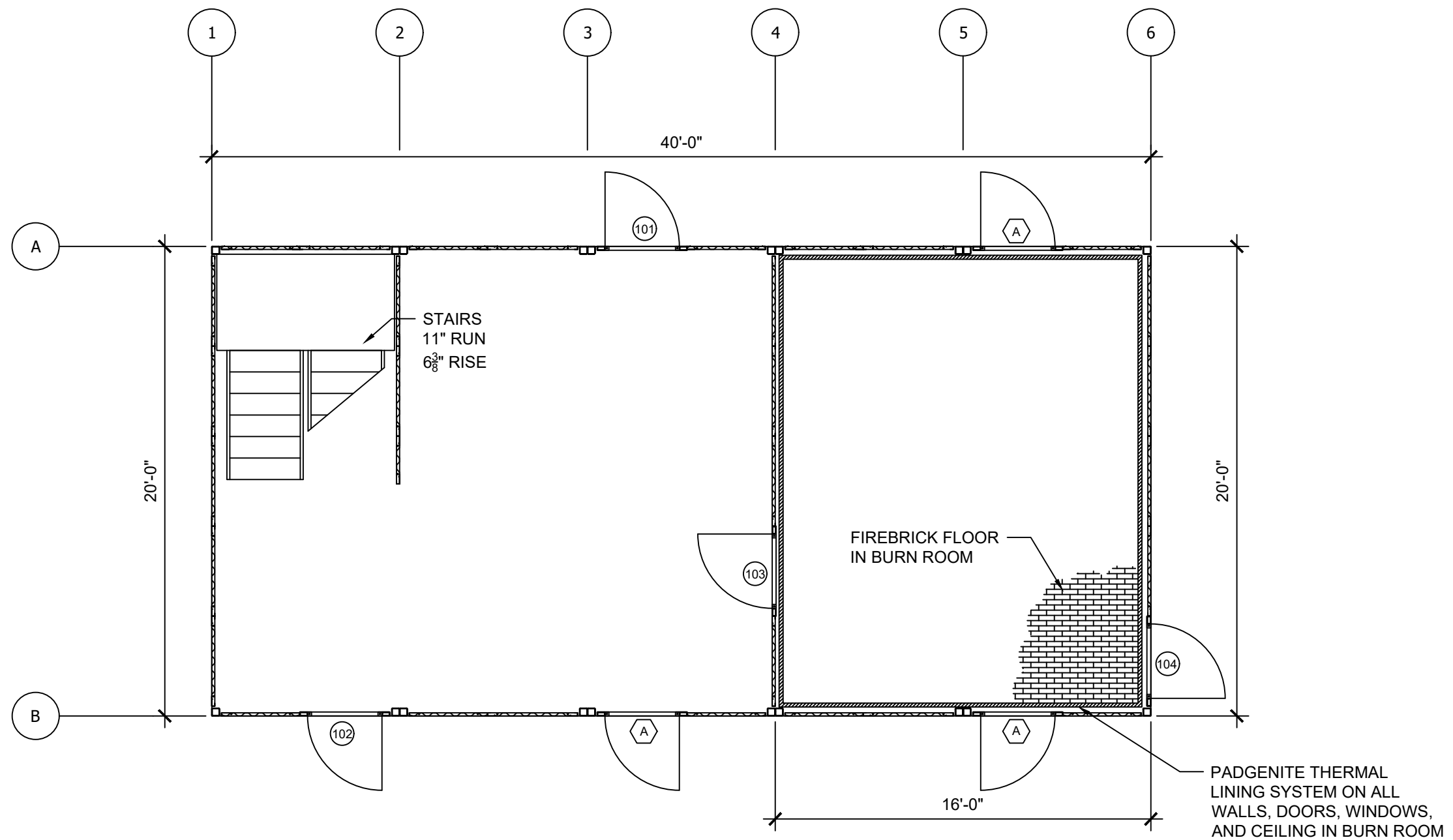
1 FIRST FLOOR LAYOUT Scale: NTS
