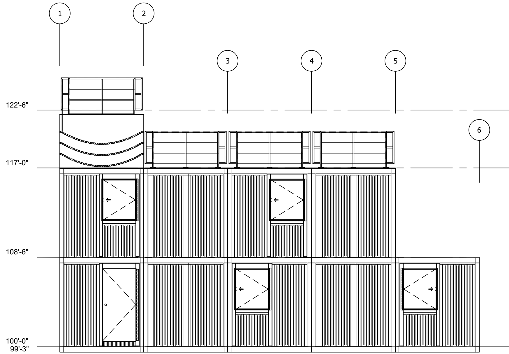
A FRONT SIDE ELEVATION Scale: NTS
