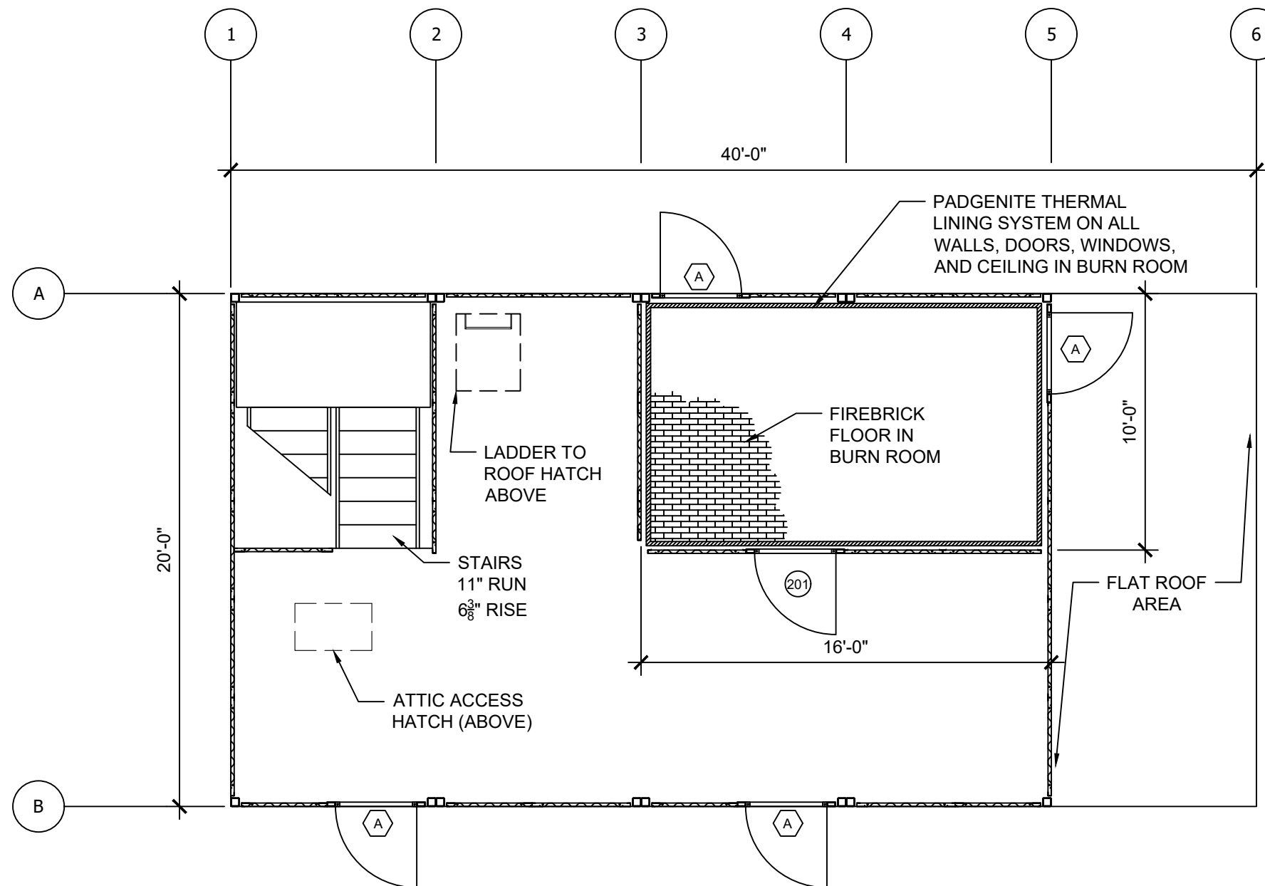
2 SECOND FLOOR LAYOUT Scale: NTS
