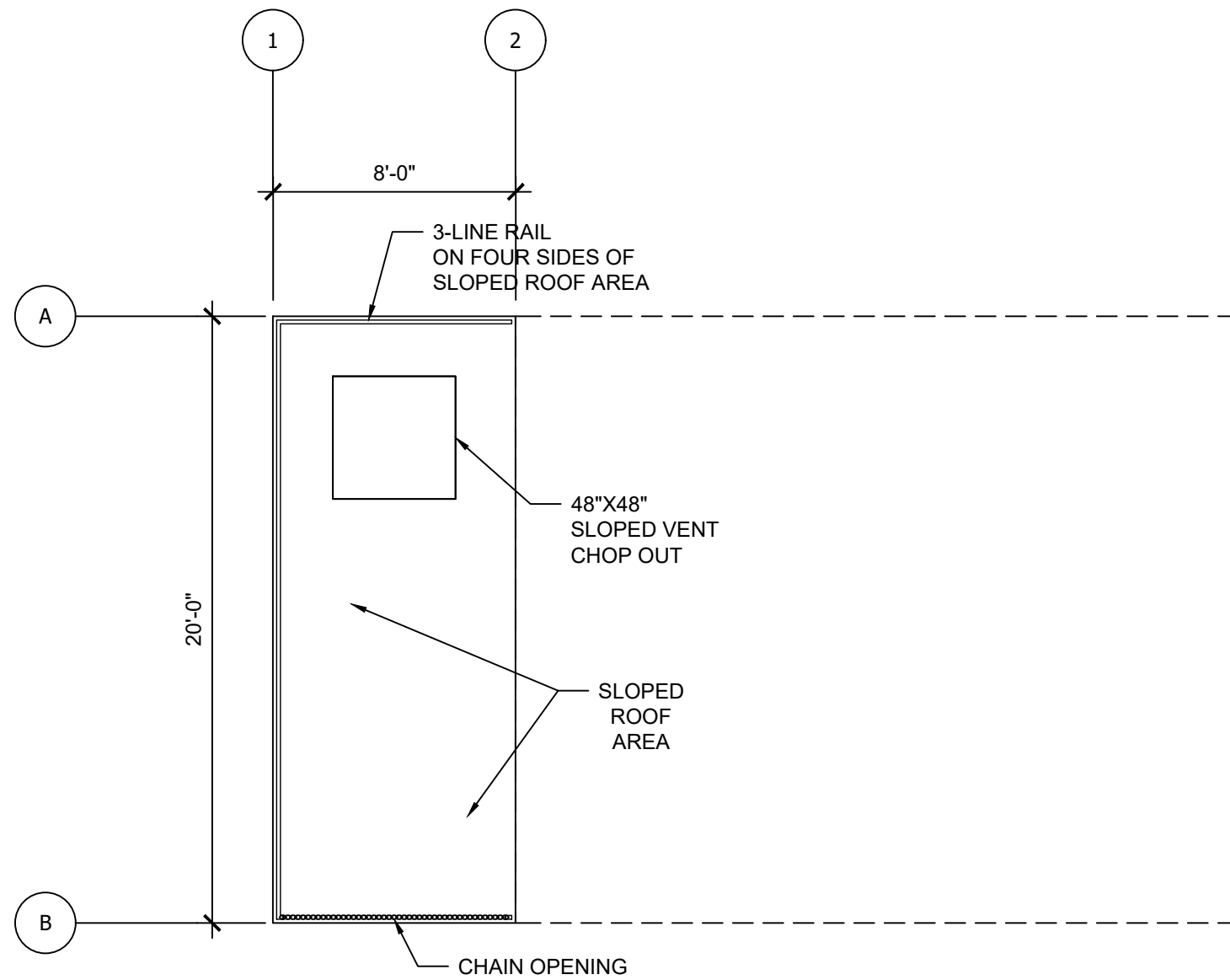
4 SLOPED ROOF LAYOUT Scale: NTS
