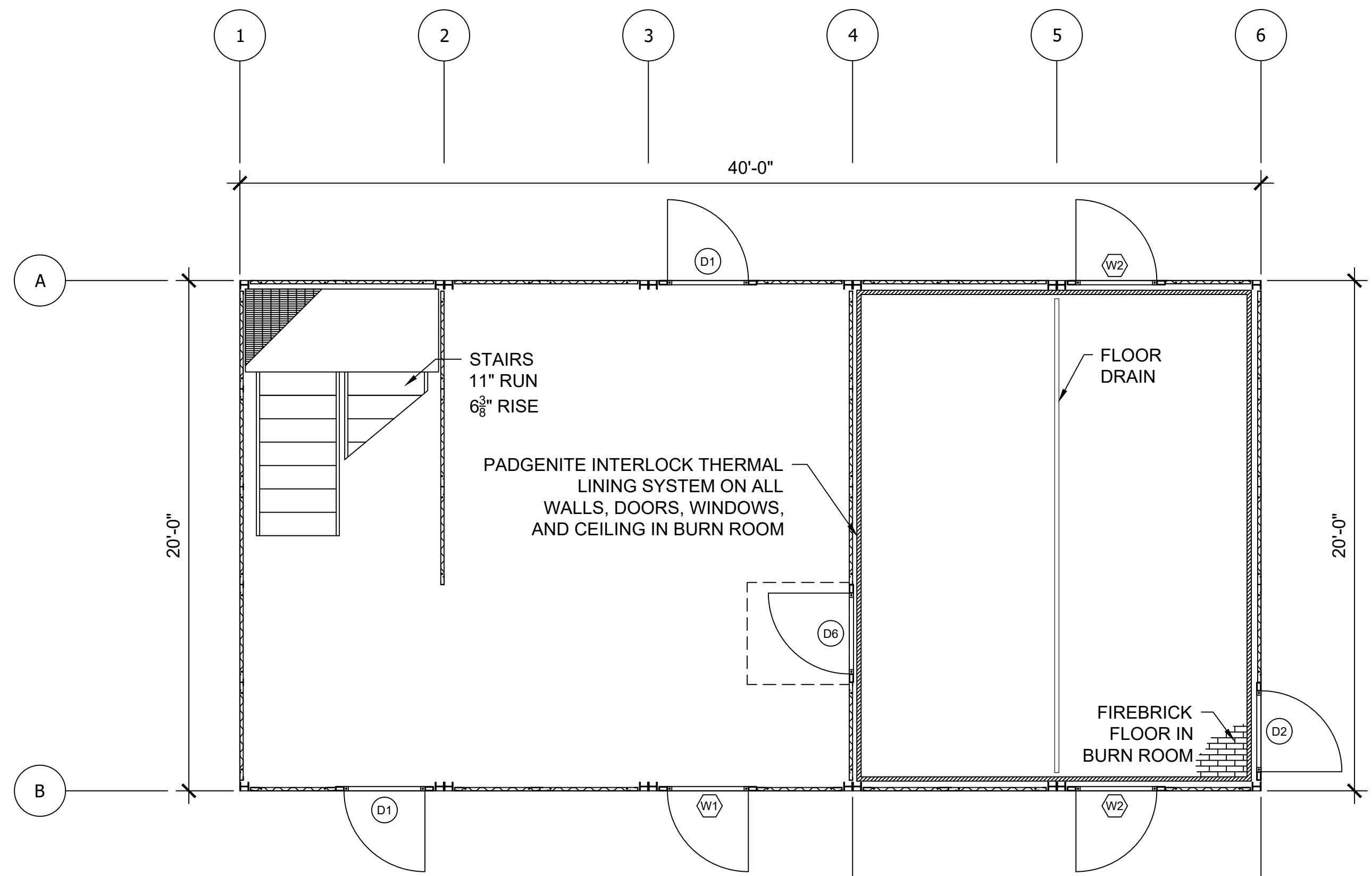
1 FIRST FLOOR LAYOUT Scale: 1/4" = 1'-0"
