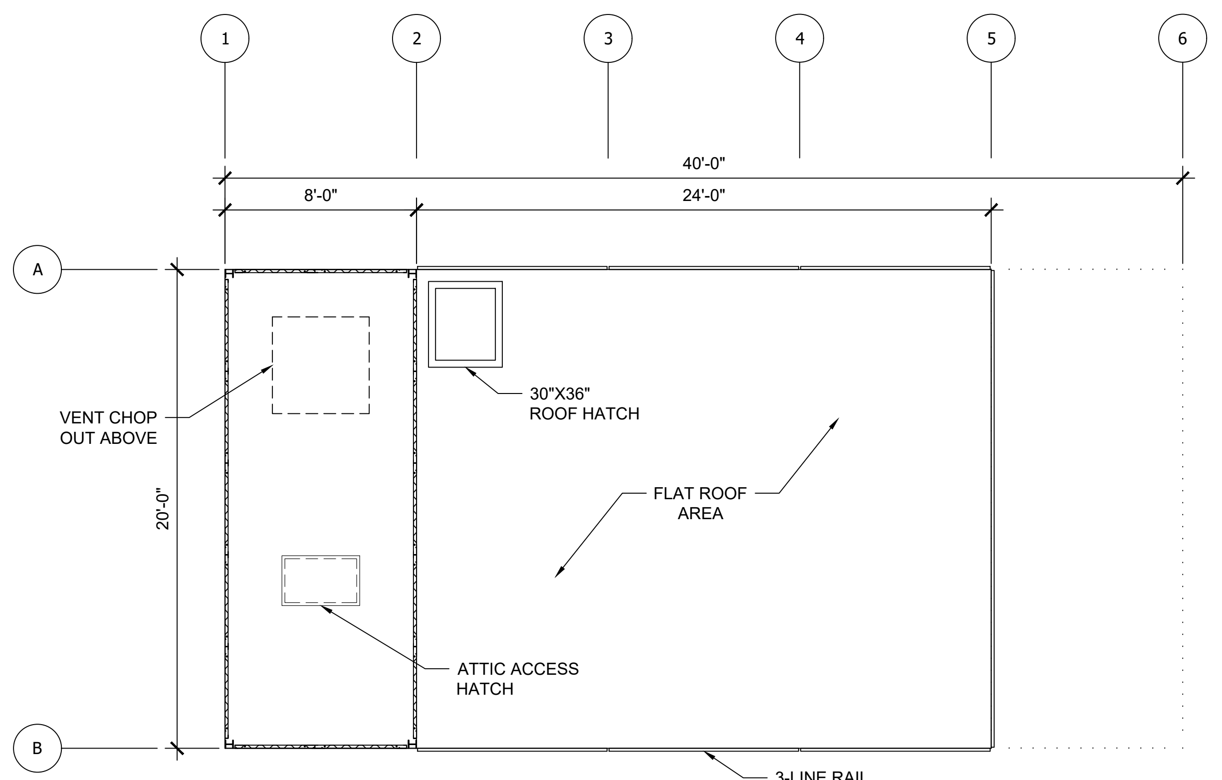
3 ROOF (ATTIC) LAYOUT Scale: 1/4" = 1'-0"
