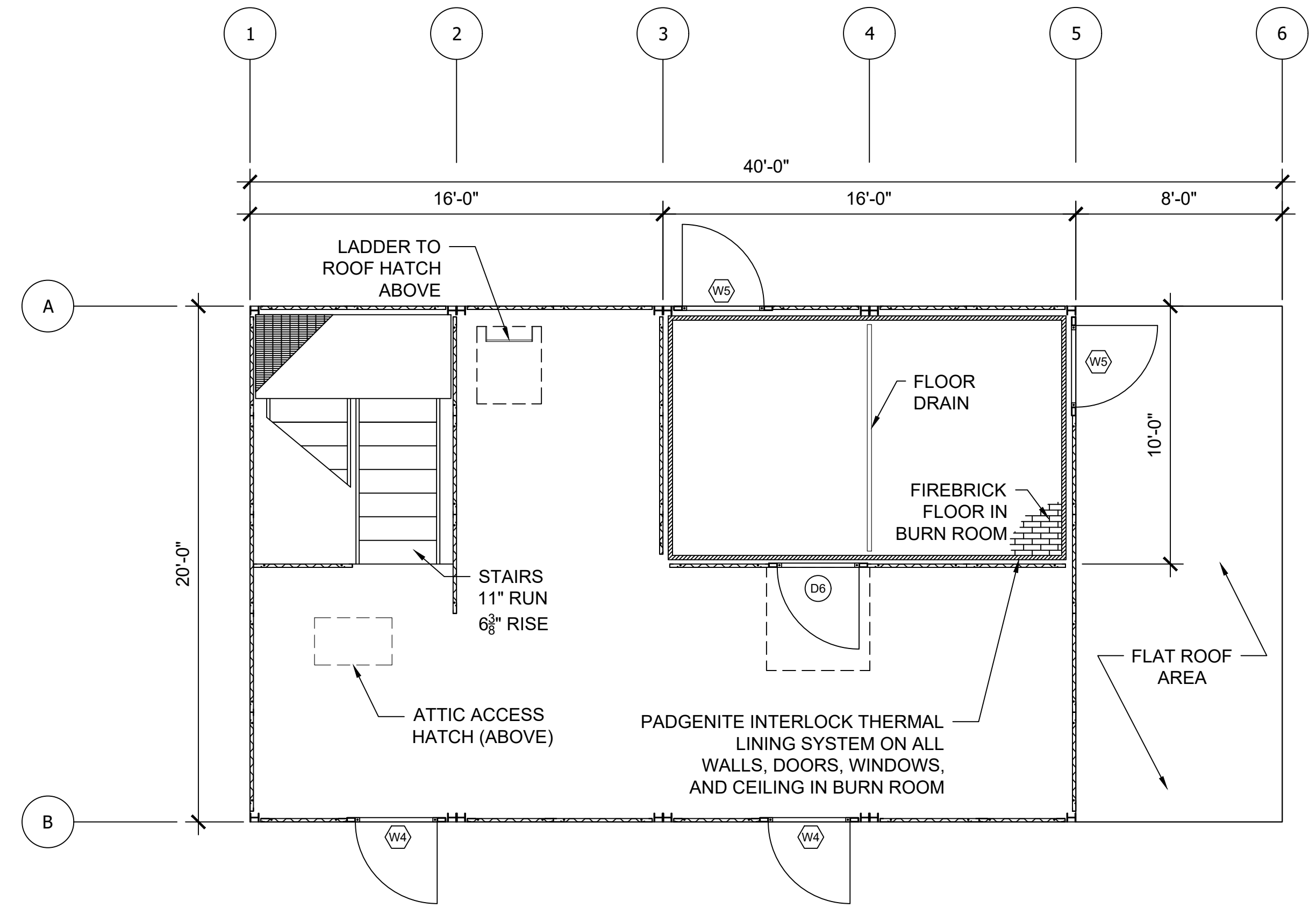
2 SECOND FLOOR LAYOUT Scale: 1/4" = 1'-0"
