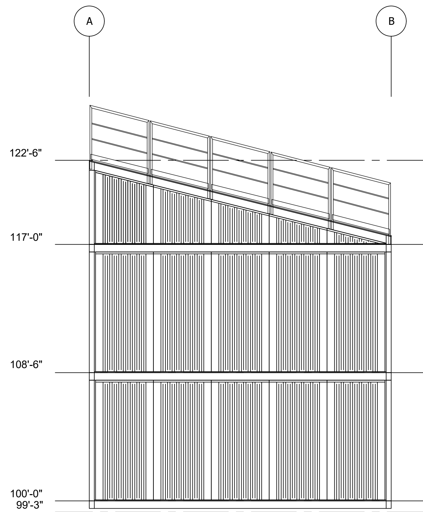
B LEFT SIDE ELEVATION Scale: 1/4" - 1'-0"
