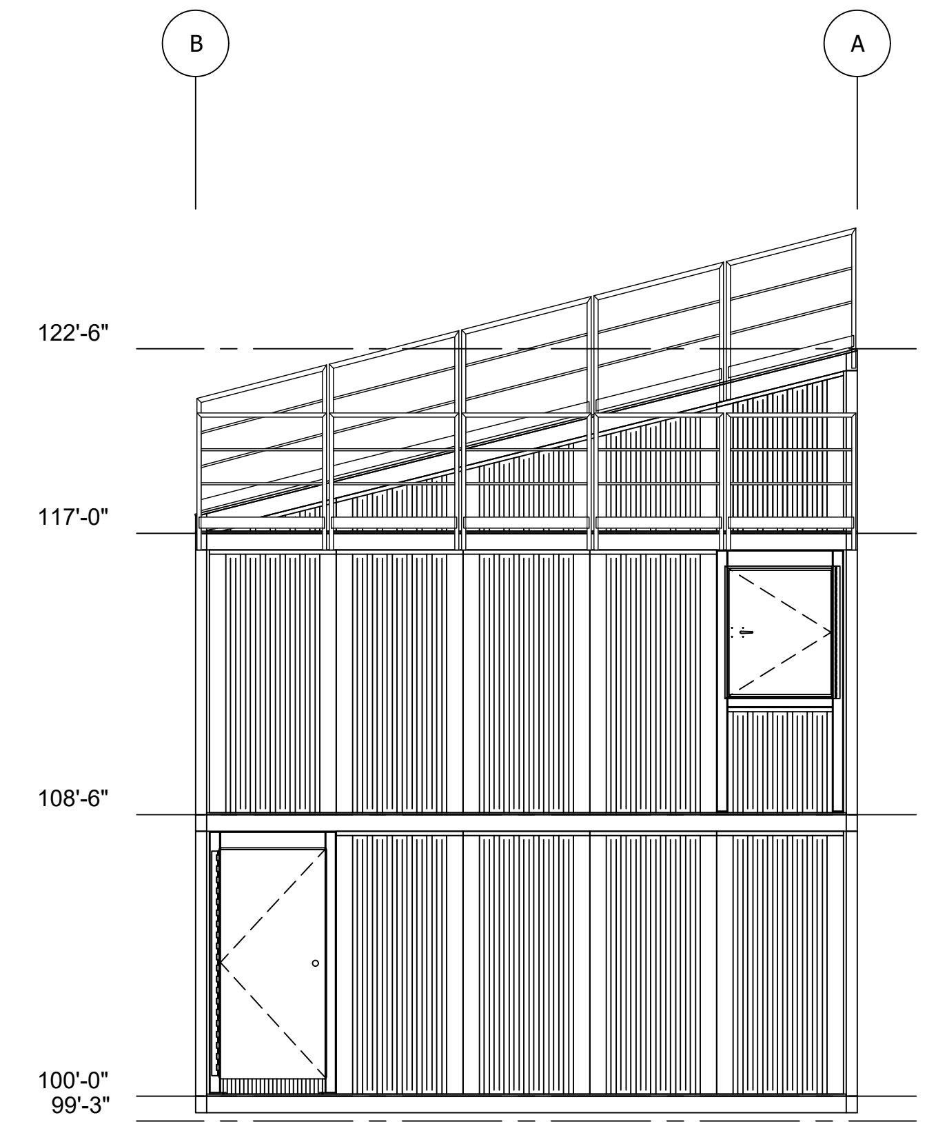
D RIGHT SIDE ELEVATION Scale: 1/4" - 1'-0"
