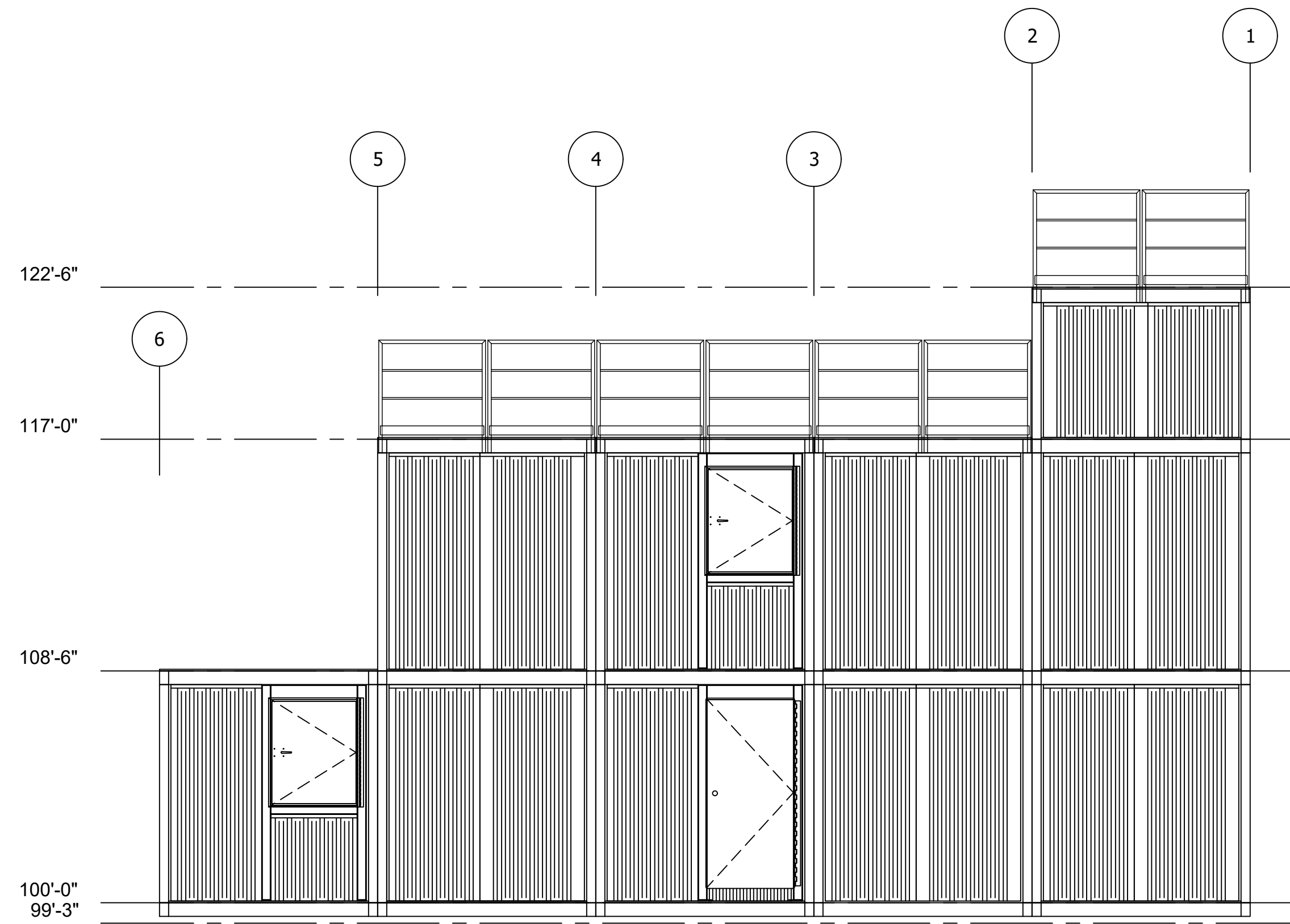
C REAR SIDE ELEVATION Scale: 1/4" - 1'-0"
