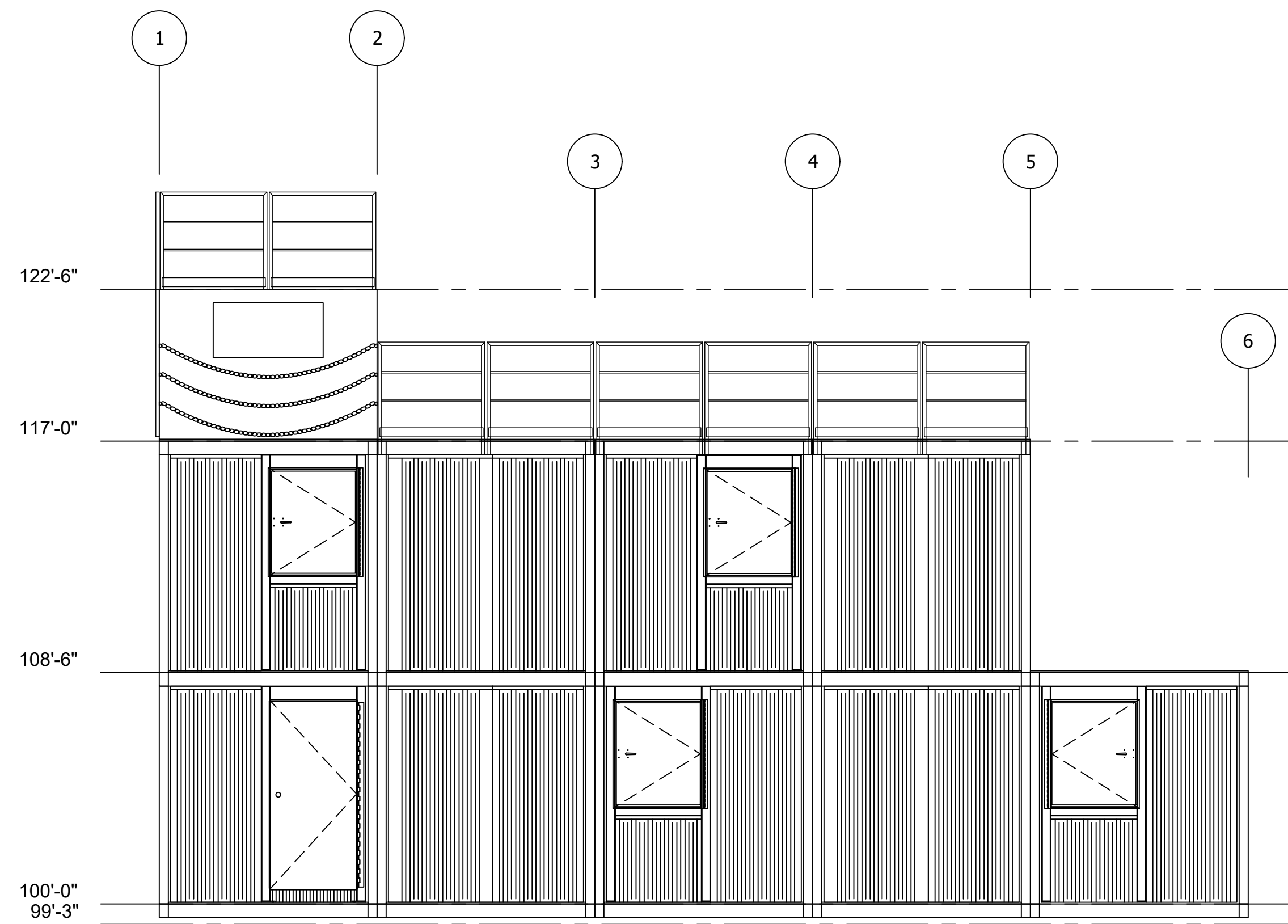
A FRONT SIDE ELEVATION Scale: 1/4" - 1'-0"
