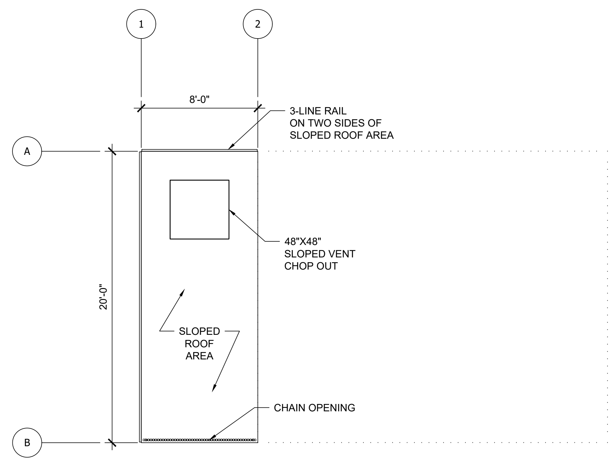
4 SLOPED ROOF LAYOUT Scale: 1/4" = 1'-0"
